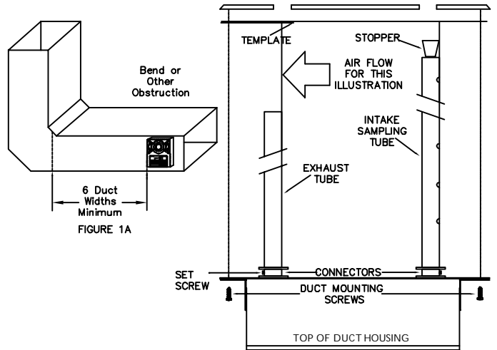
FIGURE 1B: DUCT HOUSING MOUNTING
