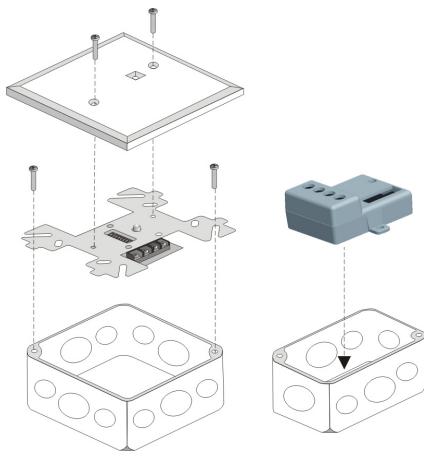
Figure 3: Mounting the SD500-AIM and SD500-MIM
