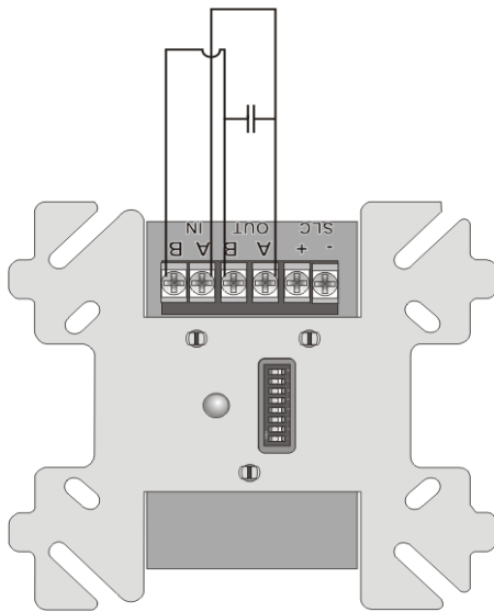
Figure 2: Class A Wiring the SD500-AIM
