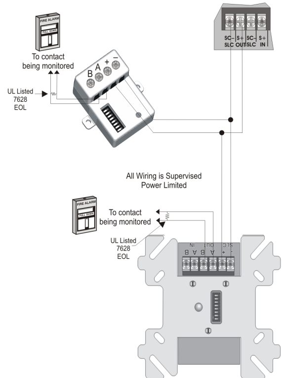
Figure 1: Class B Wiring the SD500-AIM & SD500-MIM
