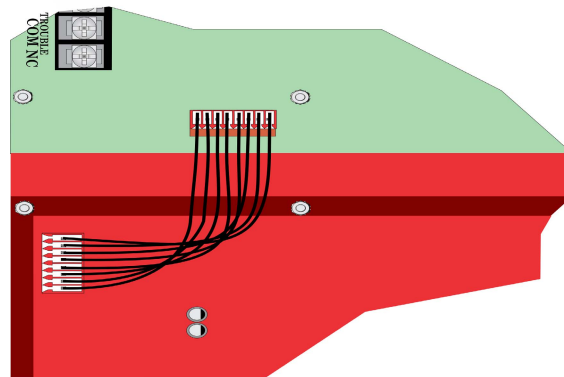
Figure 2: Wire Harness connection
