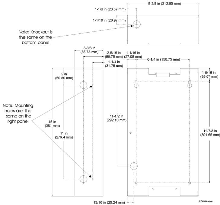
BACKBOX DIMENSIONS
