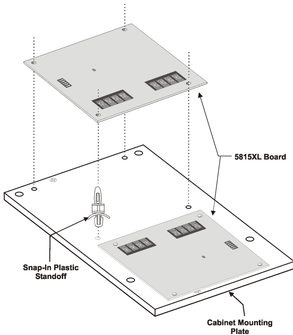
Figure 3: Standoff Installation
