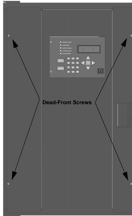
Figure 4: Plex-1 Dead-Front Installation
